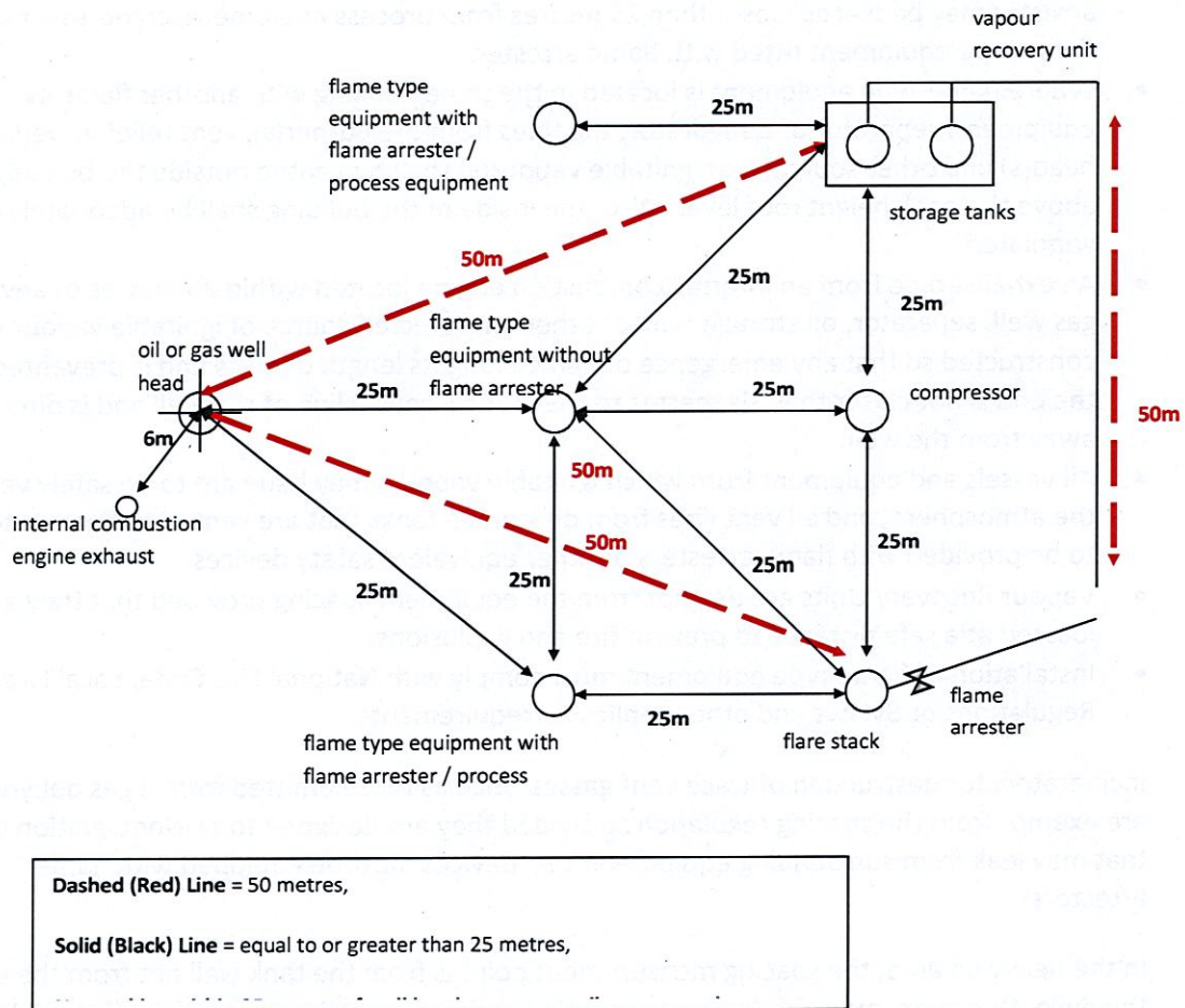
Diagram 1. Typical Equipment Spacing Diagram
